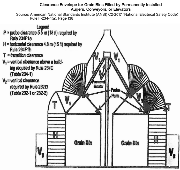
Figure 234-4(a)—Clearance envelope for grain bins filled by permanently installed augers, conveyors, or elevators
