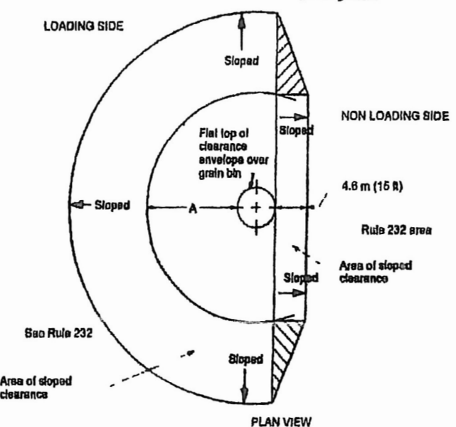
Figure 234-4(b)—Clearance envelope for grain bins filled by portable augers, conveyors, or elevators
