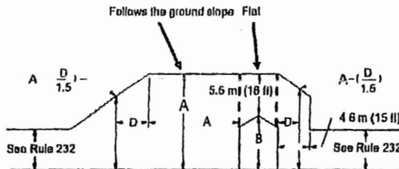
Clearance Envelope for Grain Bins Filled by Portable Augers, Conveyors, or Elevators
